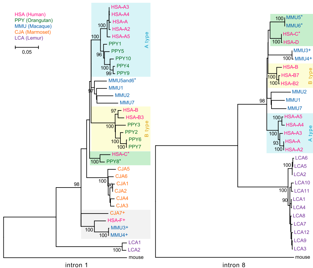
Figure 4. LRRC37 family phylogeny. Maximum likelihood phylogenetic trees were constructed using noncoding regions from intron 1 (left) and intron 8 (right). Trees are drawn to scale, with branch lengths measured in the number of substitutions per site and bootstrap values (1000 replicates) shown. Human and orangutan A- and B-type copies are shaded blue and yellow, respectively; the monophyletic clade of HSA-F paralogs is gray shaded; branches with HSA-C, HSA-D, PPY8, MMU5, and MMU6 orthologous copies are shaded green. Copies clearly mapping to syntenic locations are signed by a superscript.
