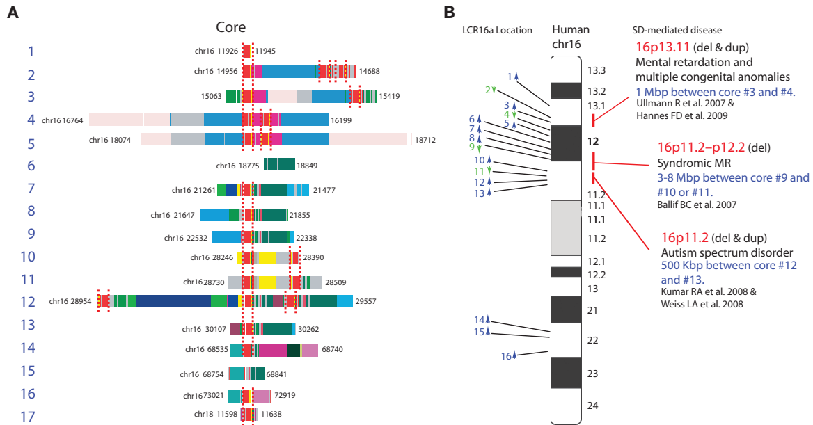
Figure 5. SDs and disease. Detailed duplication composition of duplication blocks are shown along an ideogram of human chromosome 16. Duplications mediating recurrent deletions and duplications associated with disease are indicated (Ballif et al. 2007; Jiang et al. 2007; Ullmann et al. 2007; Kumar et al. 2008; Weiss et al. 2008; Hannes et al. 2009).
