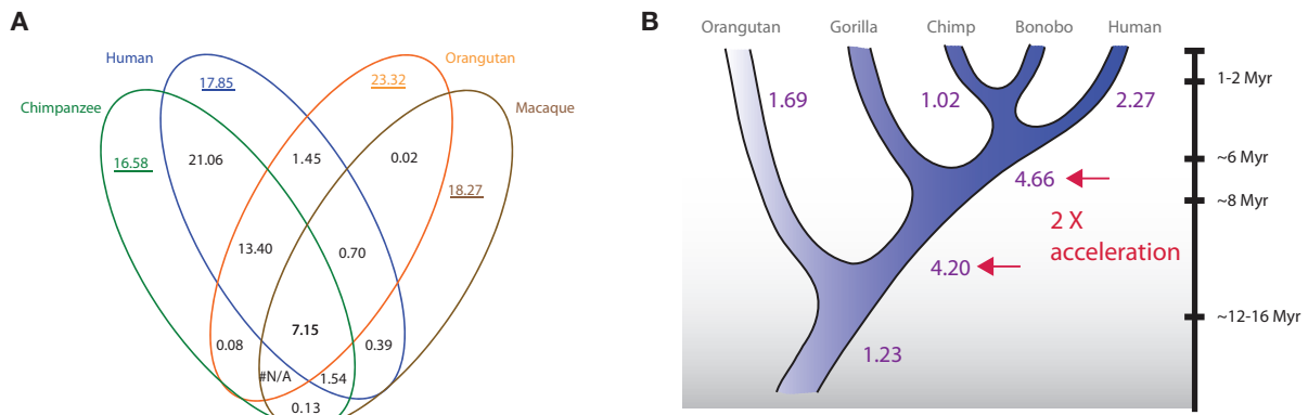
Figure 2. (A) Venn diagram showing shared and lineage-specific duplications among four primate genomes. Estimates were based on identifying regions of excess read-depth to the human assembly genome. Numbers underlined are copy-number corrected to avoid the bias of nonhuman-specific SDs. (B) Assignment of duplications and rate estimation of Mbp/Myr for each branch. Note the excess of duplication rate in the branch leading to the common ancestor of human and chimpanzee (Marques-Bonet et al. 2009).
