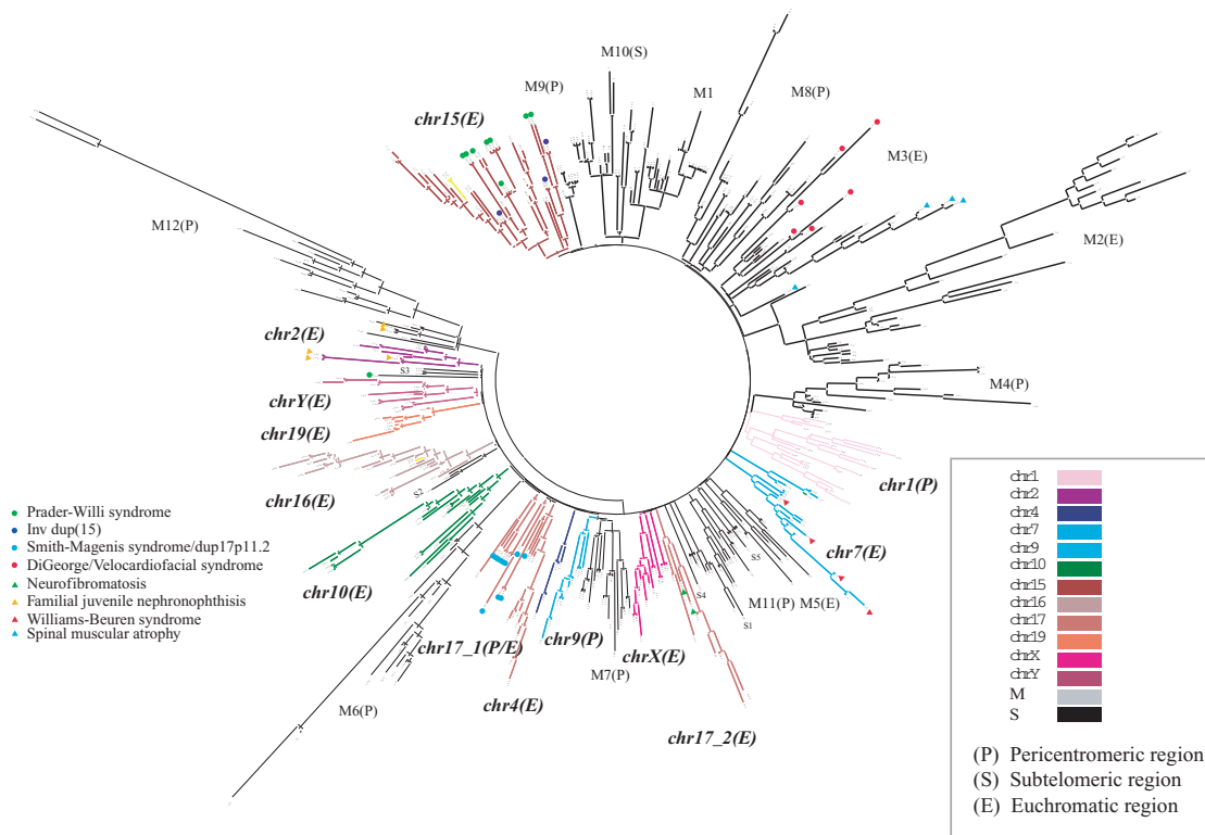
Figure 3. Hierarchical clustering of human duplication blocks based on ancestral duplicon content. The termini of each branch represent one of 437 duplication blocks, which cluster into 24 distinct groups, 14 of which are restricted to a specific chromosome and 10 of which are mixed (M) among chromosomes mapping largely to subtelomeric (S) or pericentromeric (P) regions of the genome. An expanded view of chromosome 16 is shown (Fig. 5) (Jiang et al. 2007).
