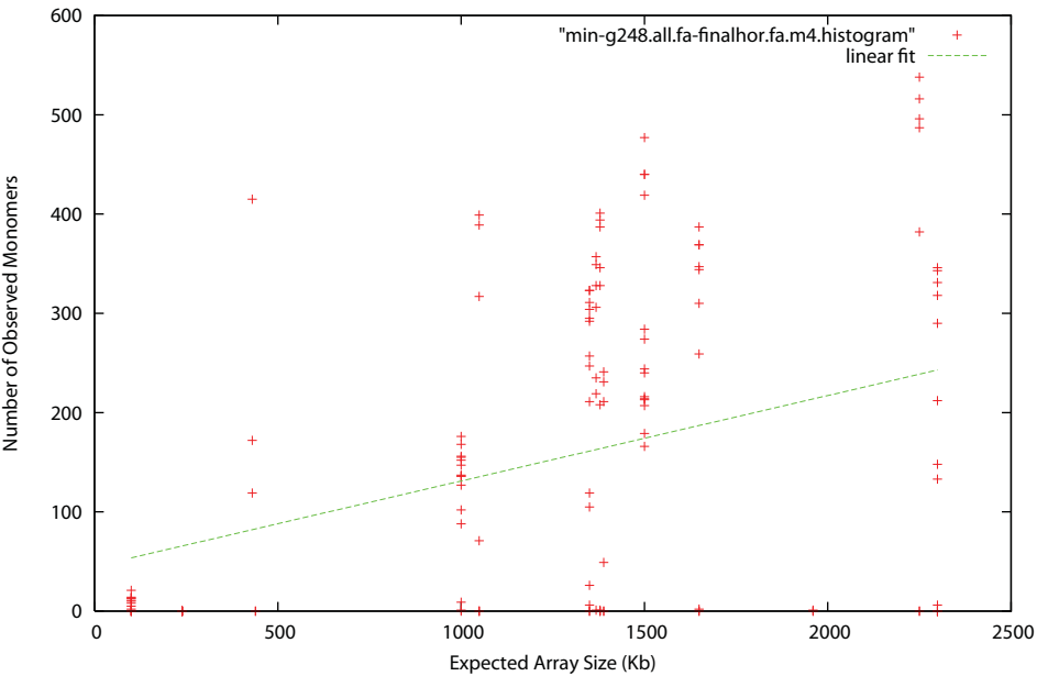
Correlation Graph of Observed Monomers vs. Minimum Expected Array Size (G248); R-Squared: 0.136603
