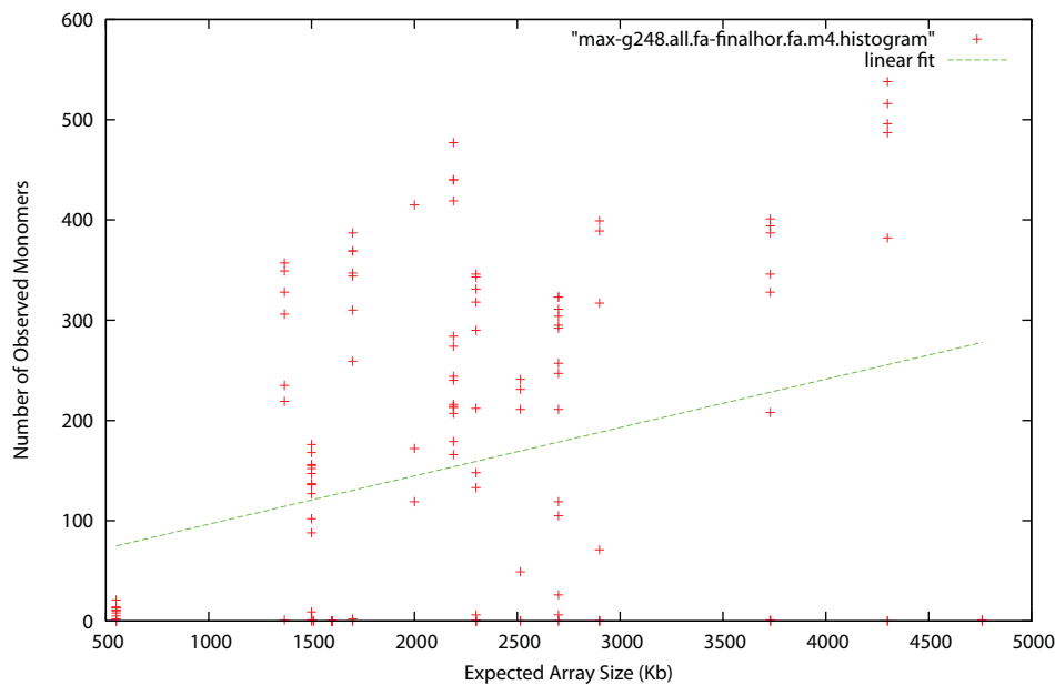
Correlation Graph of Observed Monomers vs. Maximum Expected Array Size (G248); R-Squared: 0.091203
