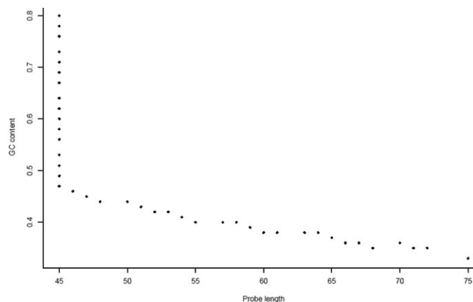
Figure 8. Probe length versus GC content. Probes with significantly greater melting temperatures than the array average appear to be GC rich probes that have been lengthened to meet a minimal threshold length of 45 bp. Deviation from this correlation at 45 bp in length reflects minimal probe length requirement of the array design.
