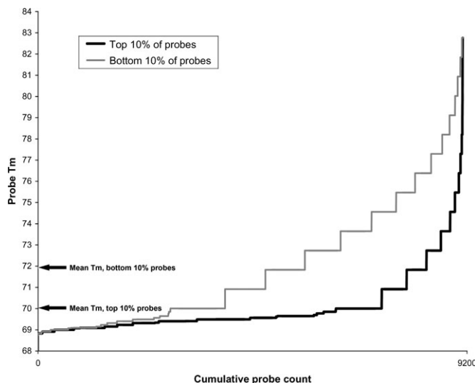
Figure 6. Relationship between probe T_m and performance. The 91 069 unique probes in the common minimal region were ranked based upon their correlation coefficient ( r ) between \log_2 ratio and DNA copy-number. In order to sample the best and worst performing probes, we utilized the top and bottom 10% tails of this distribution and the theoretical melting temperatures ( T_m ) were then plotted. Significant probe-to-probe variation in T_m is apparent. The majority of highly informative probes (those in the top 10%, all with r > 0.92 ) show a consistent isothermal distribution, with mean T_m = 70.05^\circ , standard deviation = 1.44^\circ . In contrast, the least informative probes (those in the bottom 10%, all with r < 0.3 ) show a much wider distribution which is skewed towards higher melting temperatures, with mean T_m = 71.92^\circ , standard deviation = 2.90^\circ .
