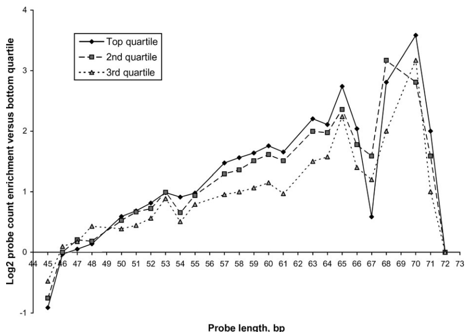
Figure 5. Probe length is correlated with probe performance. The 91 069 unique probes in the common minimal region were classified into quartiles based upon their correlation coefficient ( r ) between \log_2 ratio and DNA copy-number. The relative \log_2 enrichment of probes (lengths 45–72 bp) in the upper three quartiles versus the bottom quartile was then plotted. Probes of length 45 bp (the minimum length threshold in the array design) are 1.9-fold enriched in the bottom versus top quartile. Conversely, probes of 46 bp and above show progressively increasing enrichment in the upper quartiles, with probes of length 65 bp showing a 6.7-fold enrichment versus the bottom quartile.
