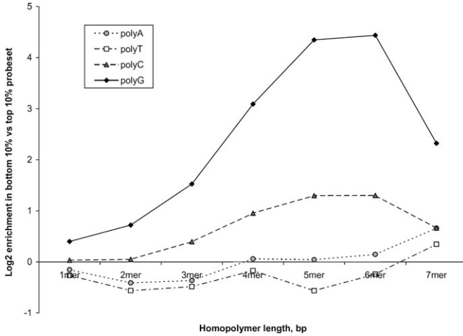
Figure 7. Differential homopolymer content influences probe performance. The 91 069 unique probes in the common minimal region were ranked based upon their correlation coefficient ( r ) between log 2 ratio and DNA copy-number. The homopolymer content (poly-A, -T, -C and -G, counting 1mers to 7mers inclusive) for all probes in the top and bottom 10% tails of r was plotted. Guanine homopolymers are significantly enriched in the least informative probes, with the motifs ‘GGGGG’ and ‘GGGGG’ occurring at >20-fold increased frequency in comparison to the most informative probes. While poly-cytosines show a milder enrichment (up to 2.5-fold for ‘CCCCC’ and ‘CCCCC’), adenine and thymine homopolymers show only small differences between the most and least informative probes (<1.6-fold difference for all polymers of ‘A’ and ‘T’).
