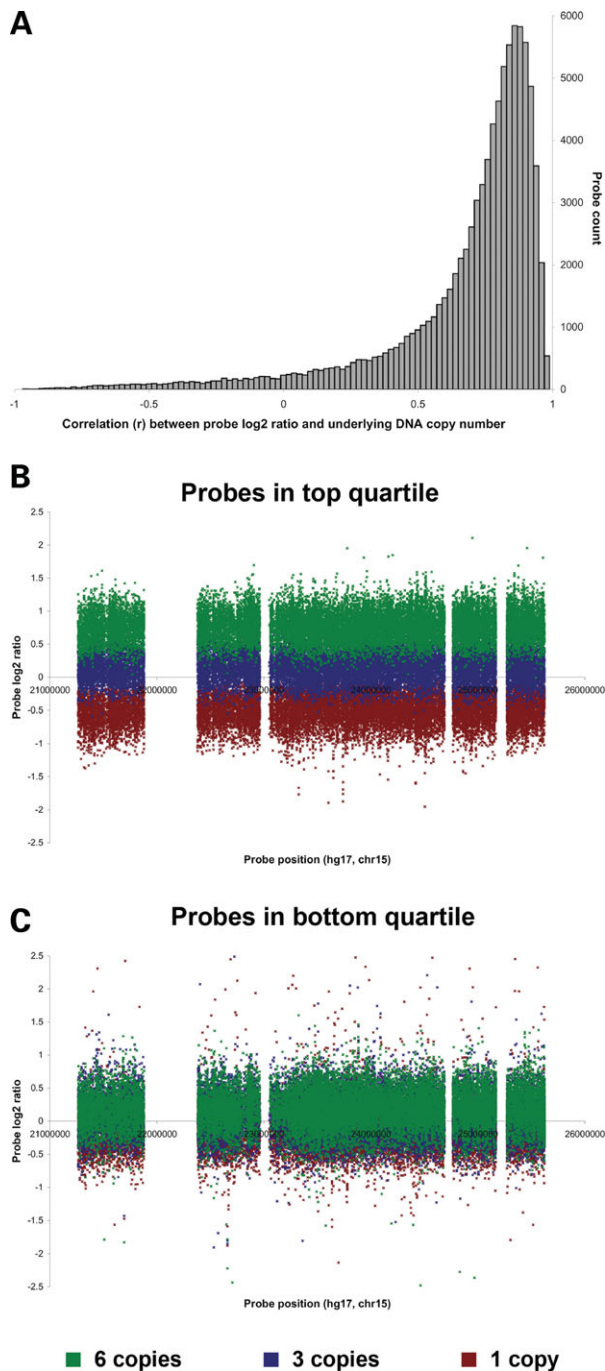
Figure 2. Correlation of individual probes with DNA copy-number is highly variable. (A) Based upon their Pearson correlation coefficient ( r ) between \log_2 ratio and DNA copy-number, each of the 91 069 unique-sequence probes were assigned into bins of width r = 0.02 . Wide variation in the data quality reported by individual probes is apparent. While some probes are highly correlated with underlying copy-number, others show a low or negative correlation. To illustrate this difference in probe performance, the 91 069 unique probes in the common minimal region were classified into quartiles based upon their correlation coefficient ( r ) between \log_2 ratio and DNA copy-number. Data for probes in the top and bottom quartiles were then plotted independently for individuals with 1, 3 and 6 copies of this region. (B) Selection of probes in the top quartile yields high-quality data in which the different DNA copy-numbers can be easily discriminated. (C) In contrast, probes in the bottom quartile of the data set (those with low or negative r -values) yield little or no useful data.
