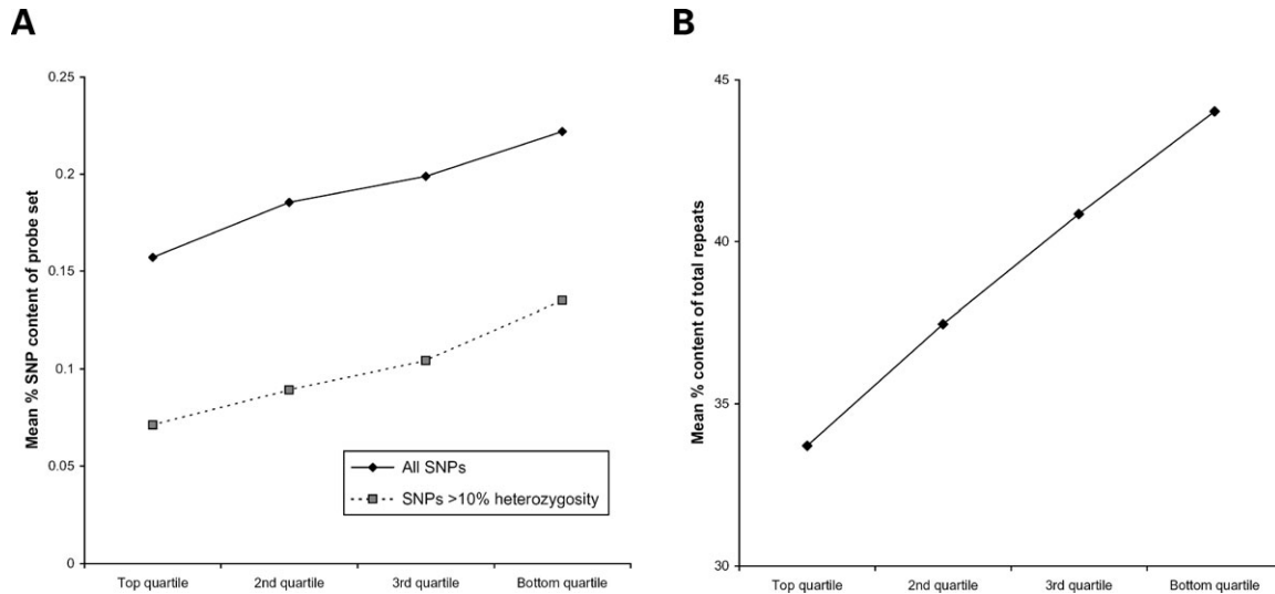
Figure 4. SNP and repetitive DNA content are inversely correlated with probe performance. Probes were classified into quartiles based upon their correlation coefficient ( r ) between \log_2 ratio and DNA copy-number. (A) SNP data were downloaded from The International HapMap Project and intersected with probe positions. The density of all SNPs, and common SNPs (defined as those with \geq 10\% minor allele frequency in the HapMap CEU population) increases as probe performance decreases. Comparing the top versus bottom quartile of probes, total SNPs are 1.4-fold enriched, while common SNPs are 1.9-fold enriched, consistent with the hypothesis that sequence polymorphism at probe binding sites adversely influences hybridization between probe and target. (B) Probe sequences were intersected with common repeats (RepeatMasker track at http://genome.ucsc.edu/ ). The density of common repeat sequences increases with decreasing probe performance. Total repeat density is 1.3-fold enriched in the top versus bottom quartile of probes.
