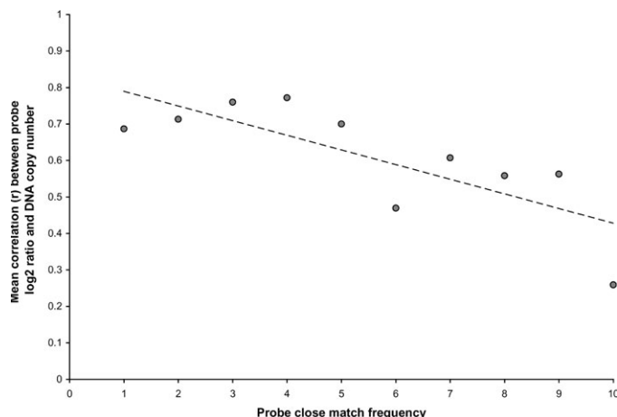
Figure 3. Non-unique probes show decreased performance. Each of the 101 013 probes in the common variant region studied (chr15:21224542–25623430) was assigned a uniqueness score. This score, termed ‘close match frequency’ (CMF) is defined as the number of locations in the genome which match the probe sequence, allowing for \leq 5 bp of insertion, deletion or substitution between probe and target. The 91 069 probes have a CMF = 1, a further 9944 probes have CMF in the range 2–10, while sites with CMF > 10 were excluded from the array design. There is an inverse correlation ( R^2 = 0.6033 ) between probe performance ( r ) and CMF, indicating that unique probes are more informative than those which hybridize to multiple genomic loci.
