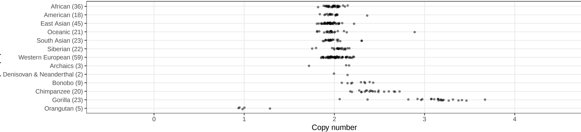
FOLH1_chr11:49145092-49208638_63546_hg38_hgdp_sunk
