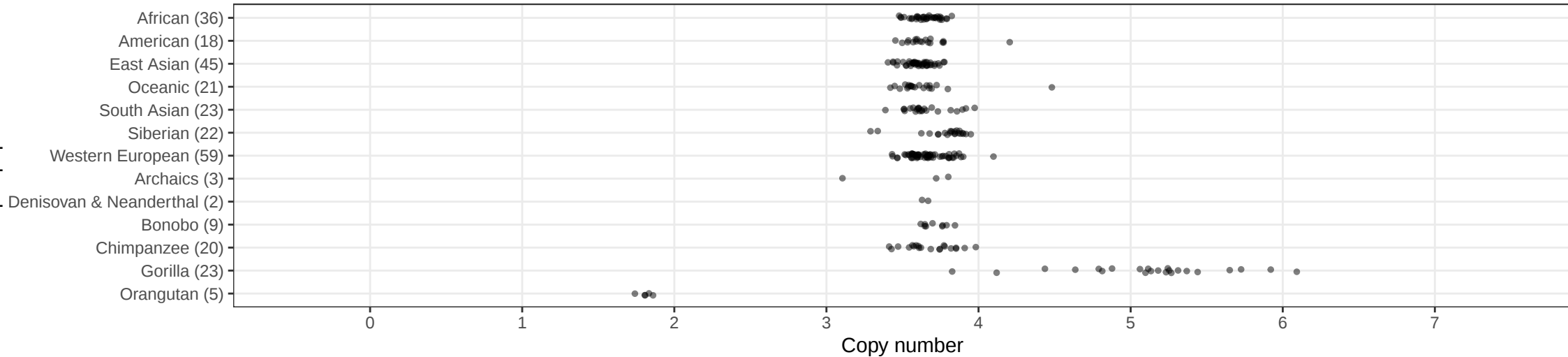
FOLH1_chr11:49145092-49208638_63546_hg38_hgdp_wssd
