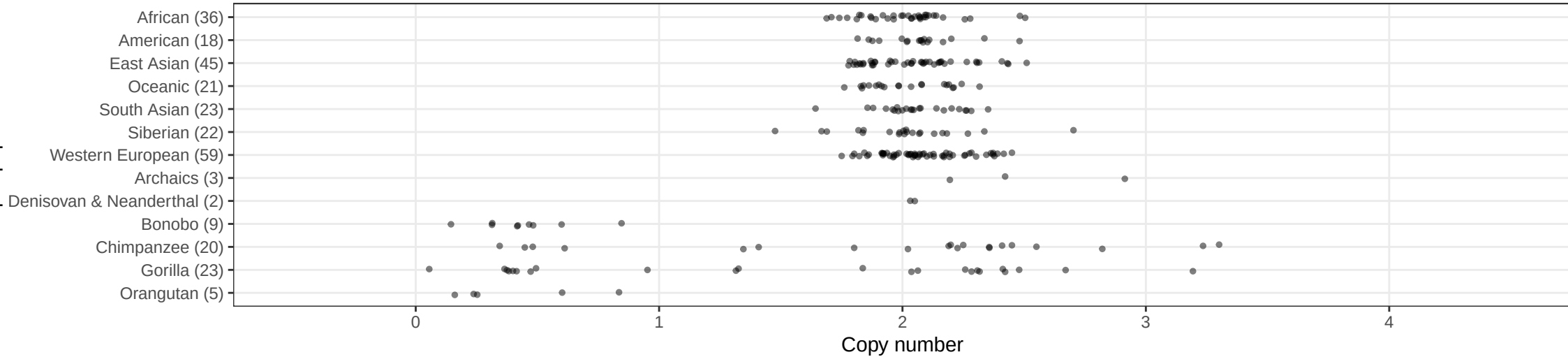
PTH2_chr19:49422419-49423441_1022_hg38_hgdp_wssd
